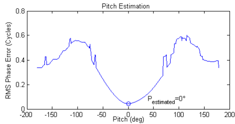
Figure 11 Pitch Estimation
