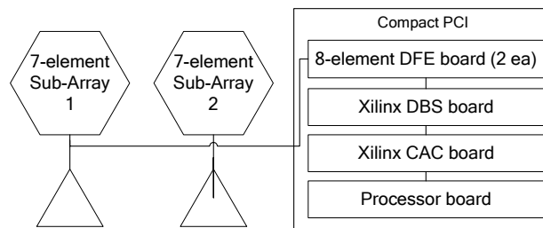
Figure 1 SSGR Design
